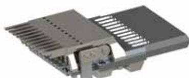
MAGAZINE ASSEMBLY, COMPLETE -#XXX (11 HOLE) CAP15CPA-XXX
