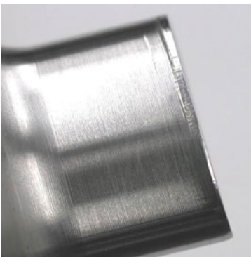
Figure 9.3. Tip damage from lack of pre-load.
