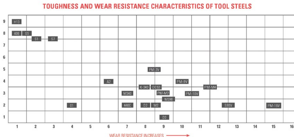
Figure 8. Toughness vs. wear resistance of various tool steels.
