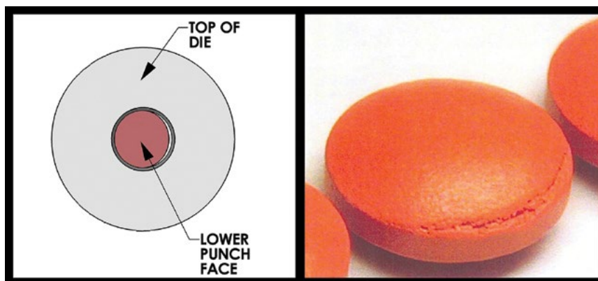
Figure 7. Off-center lower face and resulting tablet defect.
