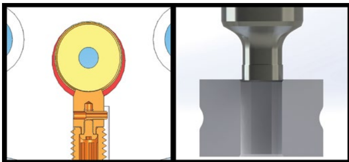
Figure 4. “Drop in” die pushed out of center by die lock screw causing tip edge contact with the lead-in chamfer of the die.
