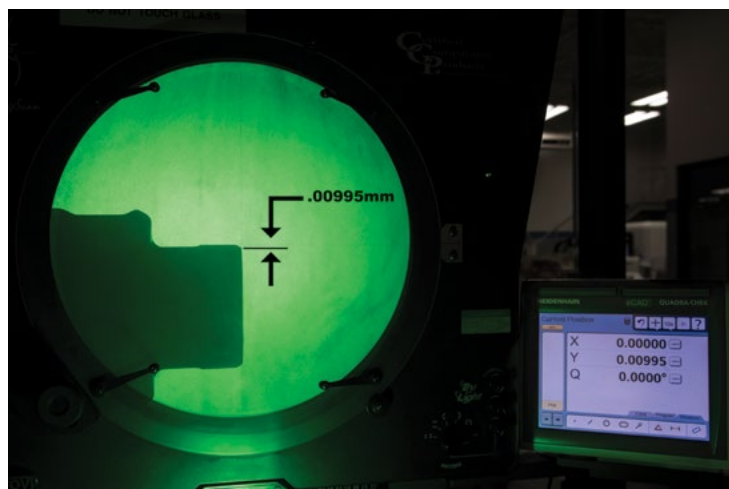
Figure 10.2. Inspection of punch tip with worn edge on optical comparator
