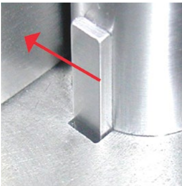
Figure 9.2. Punch key flush with left side of slot after pre-load applied (Note: these photos depict CW rotating turret).
